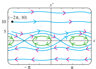
FIGURA 10.4.6 \beta = 0 .
