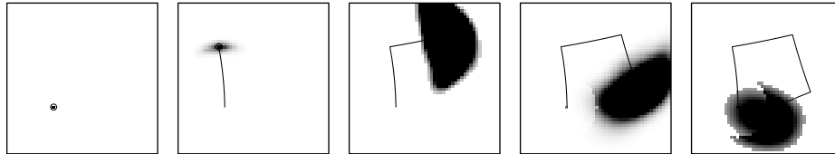
Figure 13.4 These alpha-values are based on odometry (as before) and the initial, highly uncertain map.
