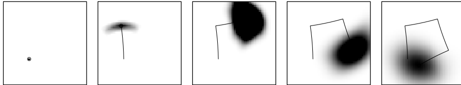
Figure 13.2 The initial alpha-values, using only odometry to compute posterior distributions over the robot's poses.
