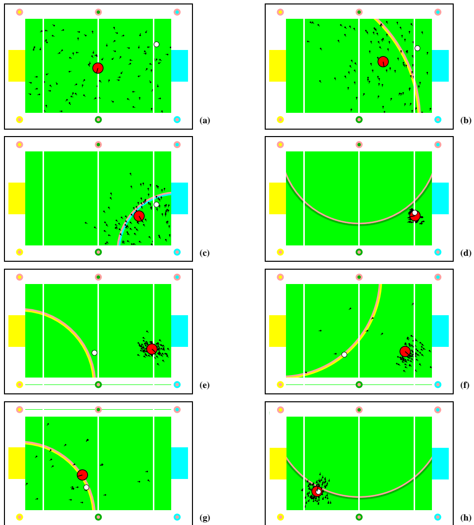
Figure 8.15 Monte Carlo localization with random particles. Each picture shows a particle set representing the robot's position estimate (small lines indicate the orientation of the particles). The large circle depicts the mean of the particles, and the true robot position is indicated by the small, white circle. Marker detections are illustrated by arcs centered at the detected marker. The pictures illustrate global localization (a)–(d) and relocalization (e)–(h).
