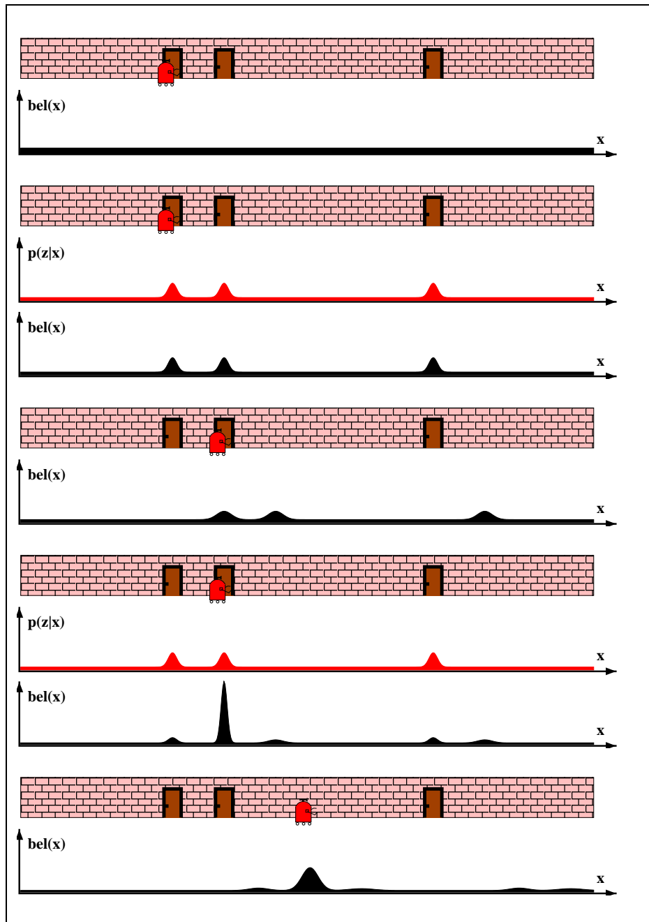
Figure 1.1 The basic idea of Markov localization: A mobile robot during global localization.
