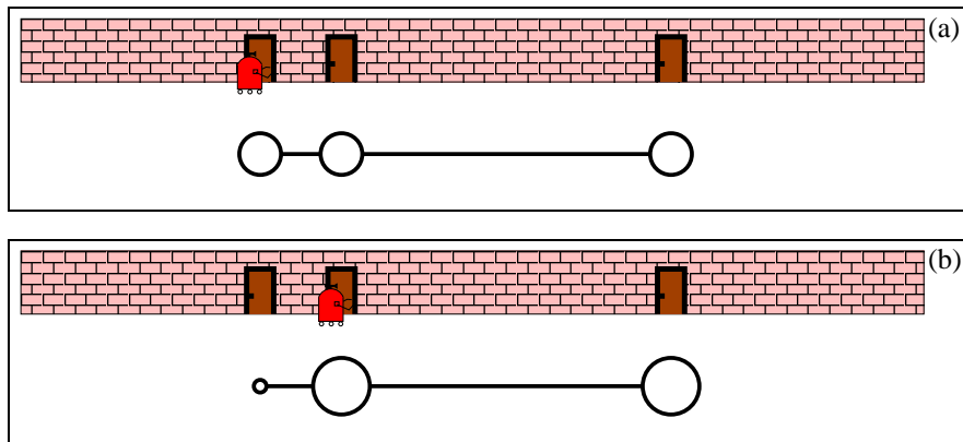
Figure 8.5 Application of a coarse-grained, topological representation to mobile robot localization. Each state corresponds to a distinctive place in the environment (a door in this case). The robot's belief bel(x_t) of being in a state is represented by the size of the circles. (a) The initial belief is uniform over all poses. (b) shows the belief after the robot made one state transition and detected a door. At this point, it is unlikely that the robot is still in the left position.
