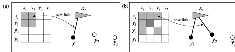
Figure 12.2 The effect of measurements on the information matrix and the associated network of features: (a) Observing y_1 results in a modification of the information matrix elements \Omega_{x_t, y_1} . (b) Similarly, observing y_2 affects \Omega_{x_t, y_2} . Both updates can be carried out in constant time.
