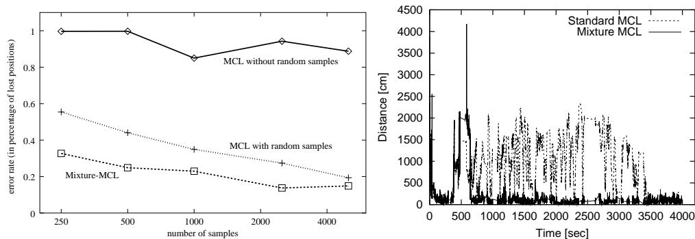
Figure 8.16 Left diagram: plain MCL (top curve), MCL with random samples (center curve), and MCL with mixture proposal distribution (bottom curve). The error rate is measured in percentage of time during which the robot lost track of its position, for a data set acquired by a robot operating in a crowded museum. Right: Error as a function of time for standard MCL and mixture MCL, using a ceiling map for localization.
