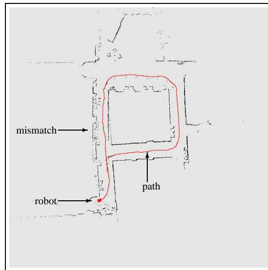
Figure 14.2 A typical map obtained using the most simple incremental maximum likelihood approach. While the map is locally consistent, the approach fails to close the cycle and leads to inconsistent maps. This elucidates the limitations of stepwise likelihood maximization, and illustrates the difficulty of mapping cyclic environments.
