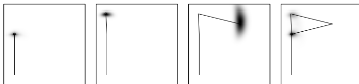
Figure 13.11 Data set 1, localization after three iterations of EM.
