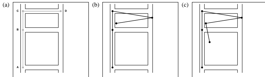
Figure 13.10 Test environment and data: (a) The environment possesses 4 indistinguishable landmark locations, labeled A to D. The robot's path is: A-B-C-D-C-B. (b) First data set, as measured by robot's odometry. (c) Second data set, which contains one more step than the first.
