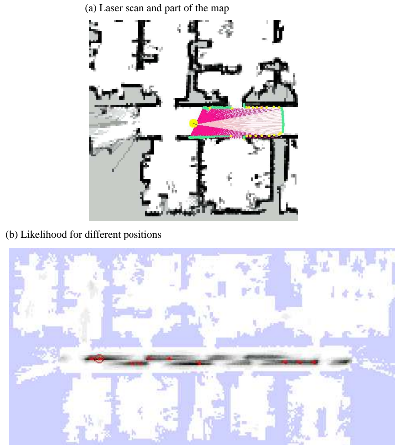
Figure 6.6 Probabilistic model of perception: (a) Laser range scan, projected into a previously acquired map m . (b) The likelihood p(z_t | x_t, m) , evaluated for all positions x_t and projected into the map (shown in gray). The darker a position, the larger p(z_t | x_t, m) .
