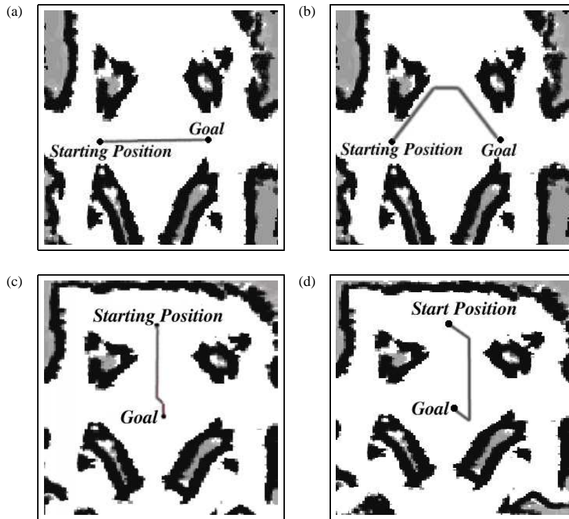
Figure 16.5 Examples of robot paths in a large, open environment, for two different configurations (top row and bottom row). The diagrams (a) and (c) are paths generated by a conventional dynamic programming path planner that ignores the robot's perceptual uncertainty. The diagrams (b) and (d) are obtained using the augmented MDP planner, which anticipates uncertainty and avoids regions where the robot is more likely to get lost. In analogy to ships who often stay close to the shore for orientation, the augmented MDP planner is known as 'coastal planner.'
