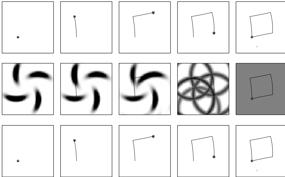
Figure 13.8 The combined results of forward and backward localization.
