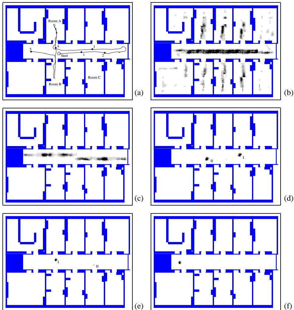
Figure 8.7 Global localization in an office environment using sonar data. (a) Path of the robot. (b) Belief as the robot passes position 1. (c) After some meters of robot motion, the robot knows that it is in the corridor. (d) As the robot reaches position 3 it has scanned the end of the corridor with its sonar sensors and hence the distribution is concentrated on two local maxima. While the maximum labeled I represents the true location of the robot, the second maximum arises due to the symmetry of the corridor (position II is rotated by 180^\circ relative to position I). (e) After moving through Room A, the probability of being at the correct position I is now higher than the probability of being at position II. (f) Finally the robot's belief is centered on the correct pose.
