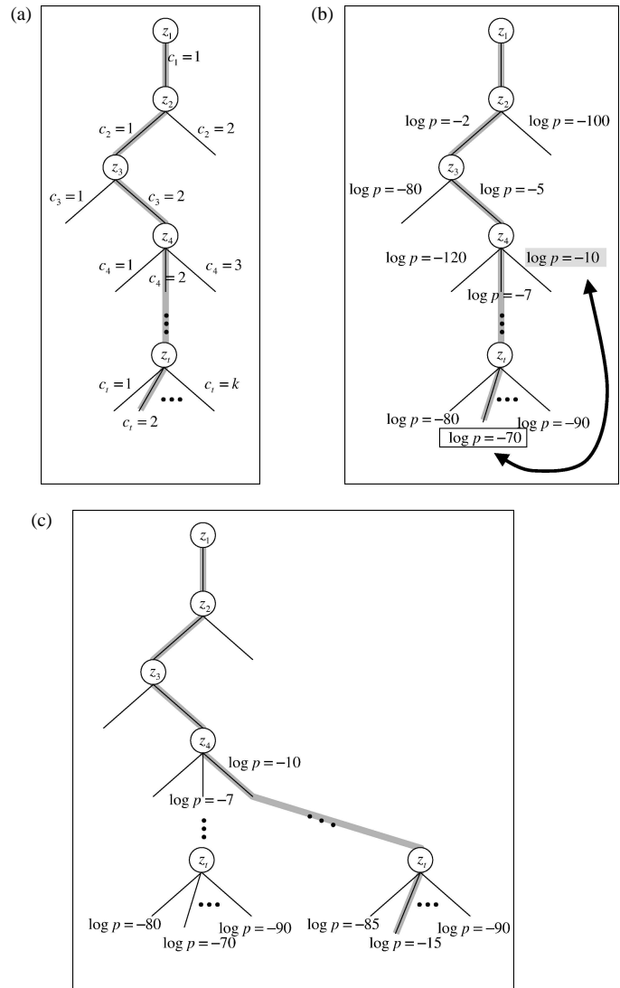
Figure 12.17 (a) The data association tree, whose branching factor grows with the number of landmarks in the map. The tree-based SEIF maintains the log-likelihood for the entire frontier of expanded nodes, enabling it to find alternative paths. (c) Improved path.
