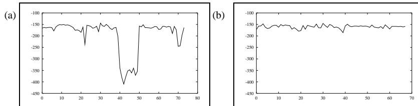
Figure 12.19 (a) Log-likelihood of the actual measurement, as a function of time. The lower likelihood is caused by the wrong assignment. (b) Log-likelihood, when recursively fitting false data association hypotheses through the tree search. The success is manifested by the lack of a distinct dip.
