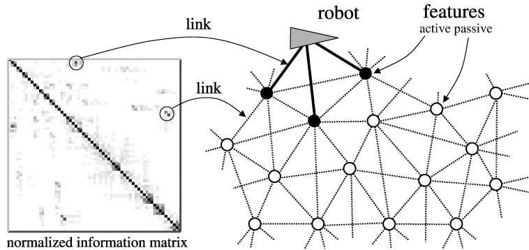
Figure 12.1 Illustration of the network of features generated by our approach. Shown on the left is a sparse information matrix, and on the right a map in which entities are linked whose information matrix element is non-zero. As argued in the paper, the fact that not all features are connected is a key structural element of the SLAM problem, and at the heart of our constant time solution.
