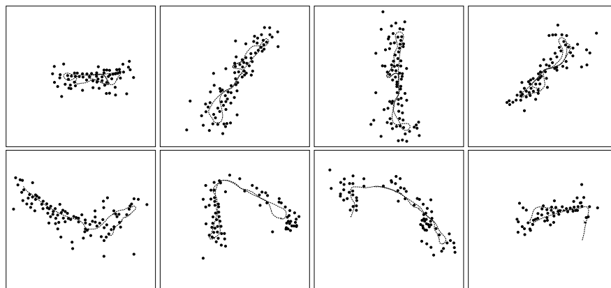
Figure 12.22 Eight local maps obtained by splitting the data into eight disjoint sequences.
