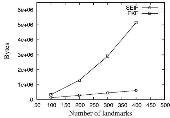
Figure 12.7 The comparison of average memory usage between SEIF and EKF.
