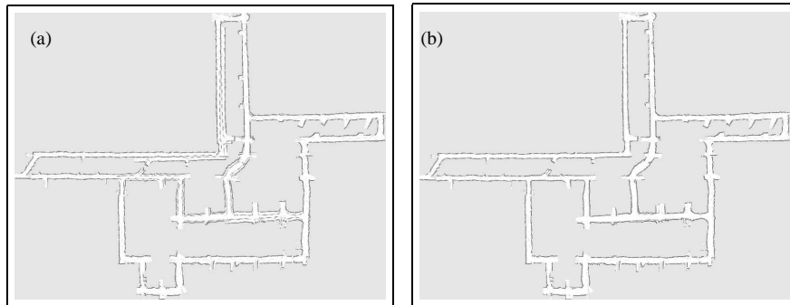
Figure 12.18 (a) Mine map with incremental ML scan matching and (b) using our lazy data association approach. The map is approximately 250 meters wide, and acquired without odometry information.
