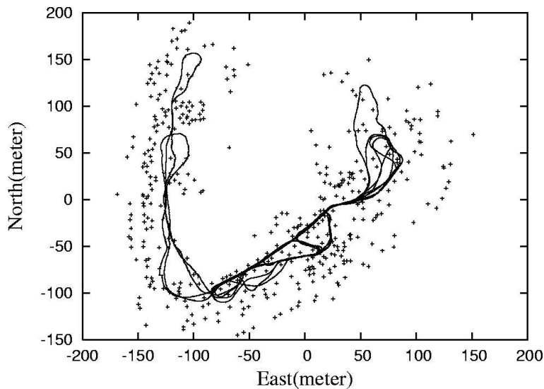
Figure 12.15 Overlay of estimated landmark positions and robot path.
