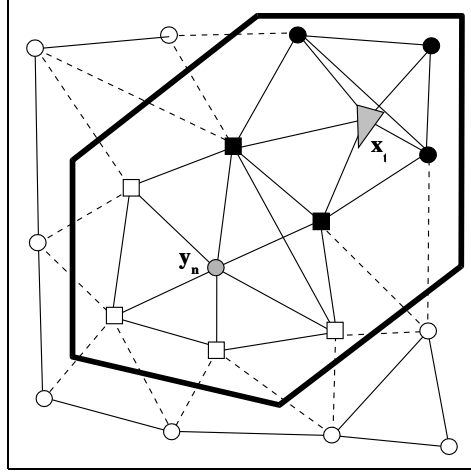
Figure 12.11 The combined Markov blanket of feature y_n and the observed features is usually sufficient for approximating the posterior probability of the feature locations, conditioning away all other features.
