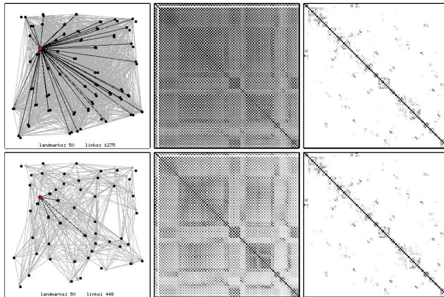
Figure 12.5 Comparison of SEIF without sparsification (top row) with SEIF with 4 active landmarks (bottom row) in a simulated environment with 50 landmarks. In each row, the left panel shows the set of links in the filter; the center panel the correlation matrix; and the right panel the normalized information matrix. Obviously, the sparsified SEIF maintains many fewer links, but its result is less confident as indicated by its less-expressed correlation matrix.
