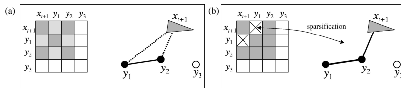
Figure 12.4 Sparsification: A feature is deactivated by eliminating its link to the robot. To compensate for this change in information state, links between active features and/or the robot are also updated. The entire operation can be performed in constant time.
