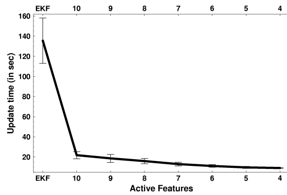
Figure 12.9 The update time of the EKF (leftmost data point only) and the SEIF, for different degrees of sparseness, as induced by a bound on the number of active features as indicated.
