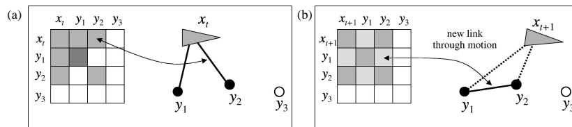
Figure 12.3 The effect of motion on the information matrix and the associated network of features: (a) before motion, and (b) after motion. If motion is non-deterministic, motion updates introduce new links (or reinforce existing links) between any two active features, while weakening the links between the robot and those features. This step introduces links between pairs of features.
