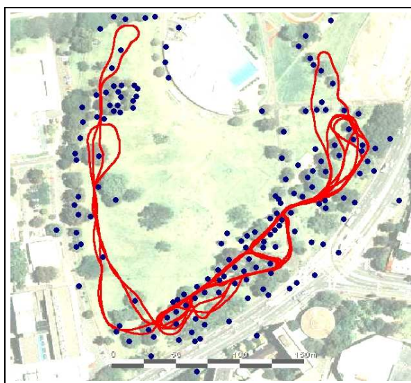
Figure 12.23 the multi-robot result, obtained using the algorithm described in this paper.
