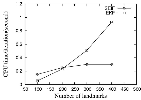
Figure 12.6 The comparison of average CPU time between SEIF and EKF.
