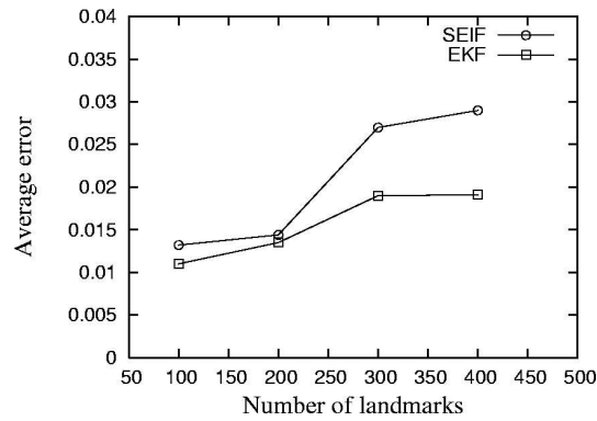
Figure 12.8 The comparison of root mean square distance error between SEIF and EKF.
