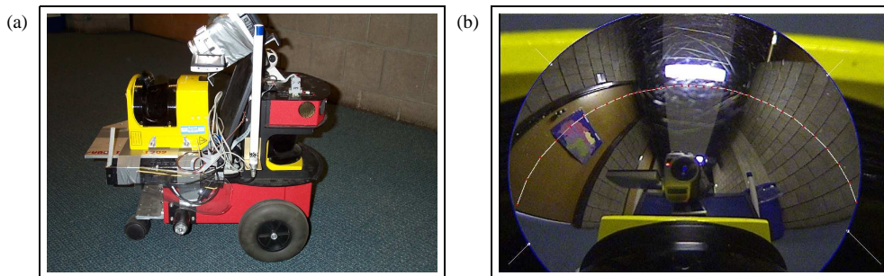
Figure 14.8 (a) Pioneer robot equipped with 2 laser range finders used for 3D mapping. (b) Panoramic image acquired by the robot. Marked here is the region in the image that corresponds to the vertical slice measured by the laser range finder.
