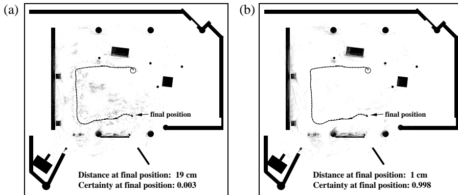
Figure 8.20 Comparison of (a) standard MCL and (b) MCL with the removal of sensor measurements likely caused by unexpected obstacles. Both diagrams show the robot path and the end-points of the scans used for localization.
