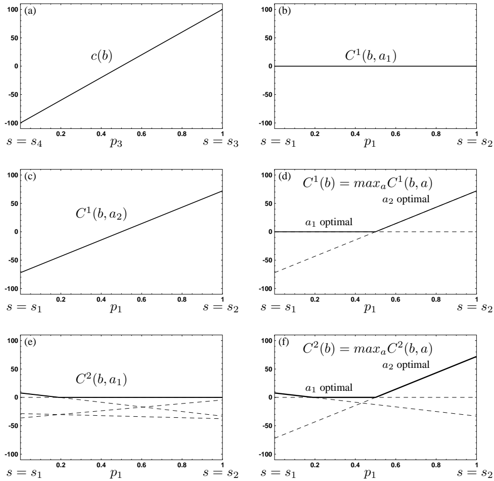
Figure 16.2 Expected payoff c(b) as a function of the belief parameter p_3 , assuming that the robot is either in state s_3 or s_4 .
