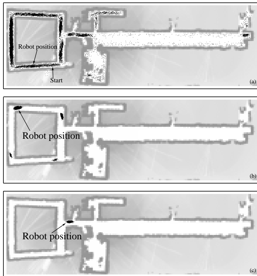
Figure 8.12 Illustration of Monte Carlo localization: Shown here is a robot operating in an office environment of size 54\text{m} \times 18\text{m} . (a) After moving 5m, the robot is still highly uncertain about its position and the particles are spread through major parts of the free-space. (b) Even as the robot reaches the upper left corner of the map, its belief is still concentrated around four possible locations. (c) Finally, after moving approximately 55m, the ambiguity is resolved and the robot knows where it is. All computation is carried out in real-time on a low-end PC.
