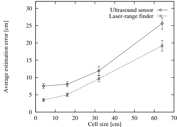
Figure 8.3 Average localization error as a function of grid cell size, for ultrasound sensors and laser range-finders.
