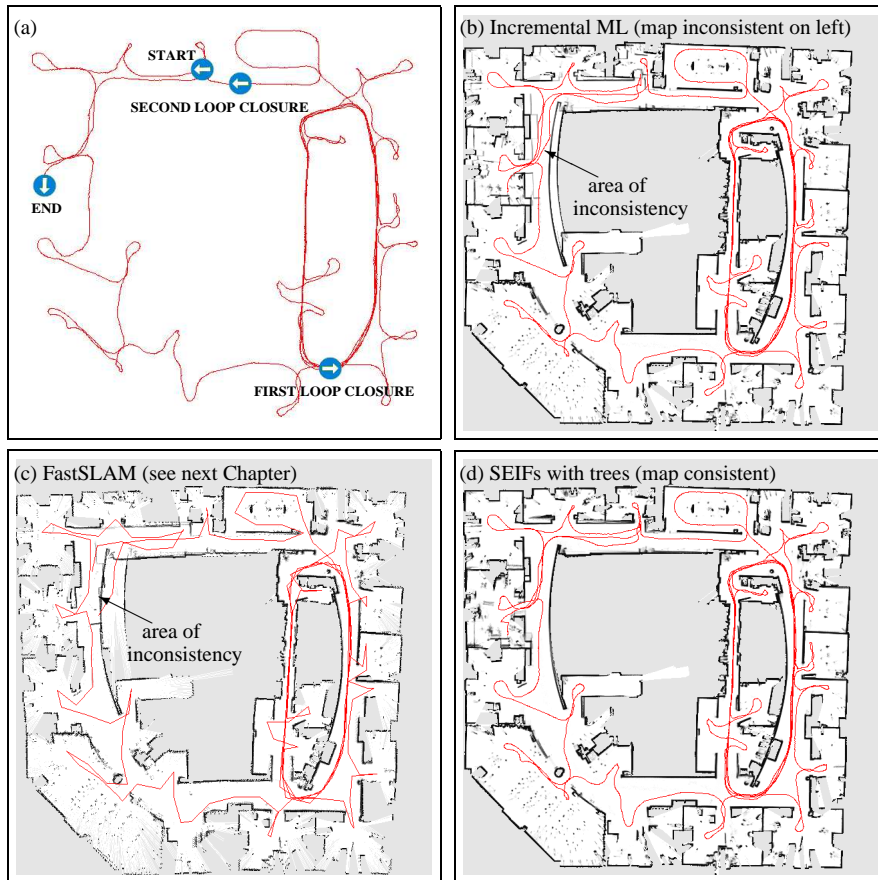
Figure 12.21 (a) Path of the robot. (b) Incremental ML (scan matching) (c) FastSLAM. (d) Our approach.
