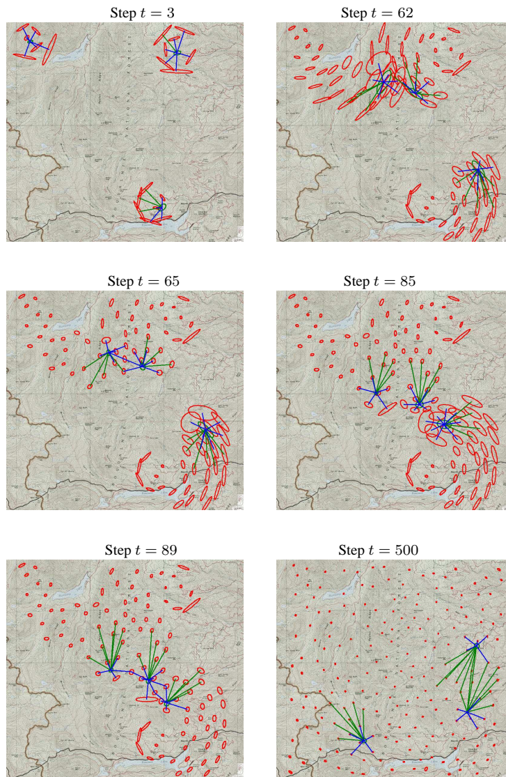
Figure 12.16 Snapshots from our multi-robot SLAM simulation at different points in time. Initially, the poses of the vehicles are known. During Steps 62 through 64, vehicle 1 and 2 traverse the same area for the first time; as a result, the uncertainty in their local maps shrinks. Later, in steps 85 through 89, vehicle 2 observes the same landmarks as vehicle 3, with a similar effect on the overall uncertainty. After 500 steps, all landmarks are accurately localized.
