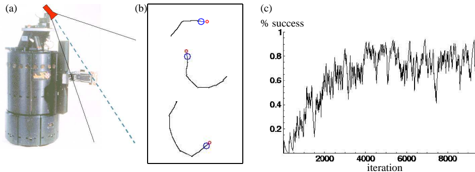
Figure 16.4 Find and fetch task: (a) The mobile robot with gripper and camera, holding the target object (experiments are carried out in simulation!), (b) three successful runs (trajectory projected into 2D), and (c) success rate as a function of number of planning steps.
