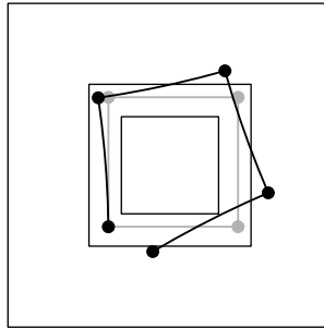
Figure 13.1 Environment (thin line); the robot's path (grey); and the measured path (thick line). The robot can perceive whether or not it is in one of the indistinguishable corners, within a certain maximum perceptual range. The dots indicate locations where the robot perceived a corner.
