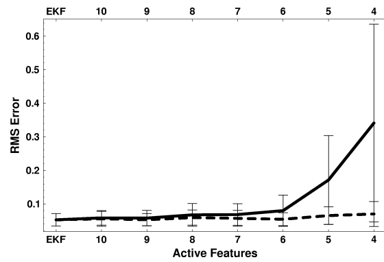
Figure 12.10 The approximation error EKF (leftmost data point only) and SEIF for different degrees of sparseness. In both figures, the map consists of 50 landmarks.
