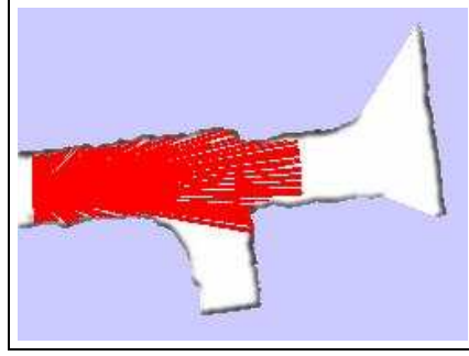
Figure 6.11 Example of a local map generated from 10 range scans, one of which is shown.
