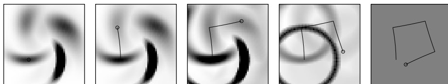
Figure 13.5 Backwards localization: The beta-values are computed from right to left, effectively localizing the robot backwards in time.
