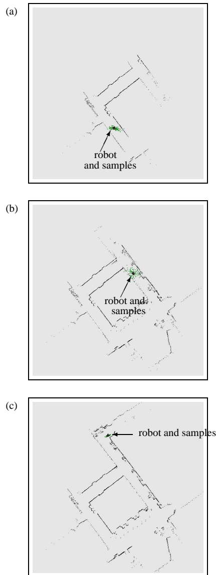
Figure 14.3 Mapping cyclic environments using particle filters for posterior pose estimation. The dots, centered around the robot, indicate the posterior belief which grows over time (a and b). When the cycle is closed as in (c), the map is revised accordingly and the posterior becomes small again.
