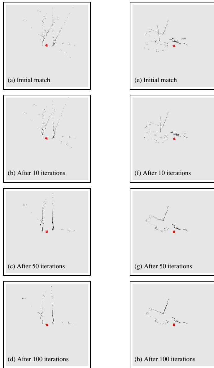
Figure 14.1 To examples of gradient descent for aligning scans (arranged vertically). In both cases, the initial translational error is 10 cm along each axis, and the rotational error is 30 degrees. The gradient descent algorithm safely recovers the maximum likelihood alignment.
