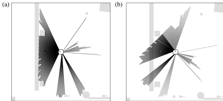
Figure 8.19 Illustration of our measurement rejection algorithm: Shown in both diagrams are range scans (no max-range readings). Lightly shaded readings are filtered out.
